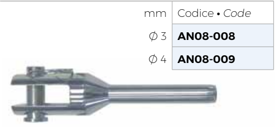
Terminale a forcella per cavo Ø 3 | 4 mm in acciaio inox AISI 316 Fork terminal for wire rope Ø 3/4mm Stainless steel AISI 316
